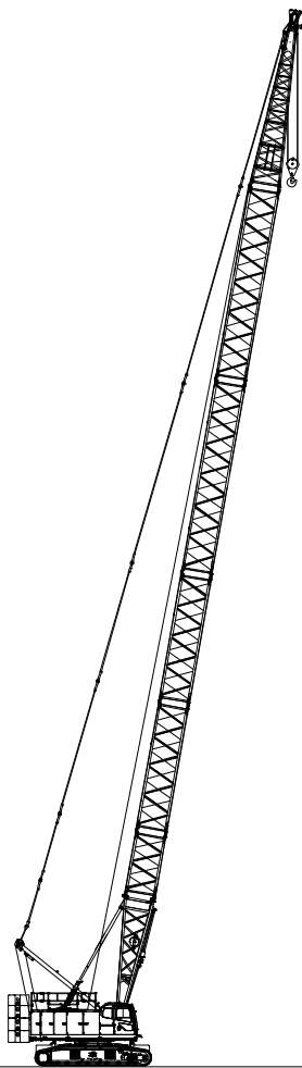
45–155 ft (13.72–47.74m) Main Angle Boom
